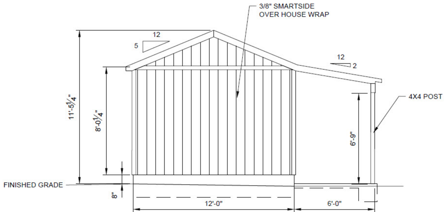
WALL A ELEVATION
